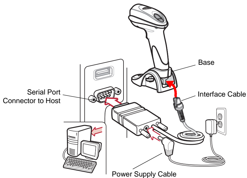
Figure 5-2 SSI Host Connection for Scanner with Base
