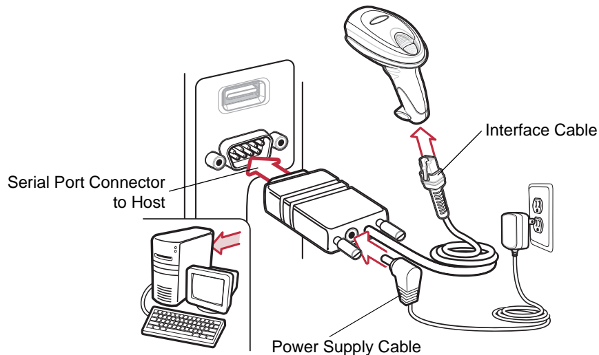
Figure 5-1 SSI Host Connection
